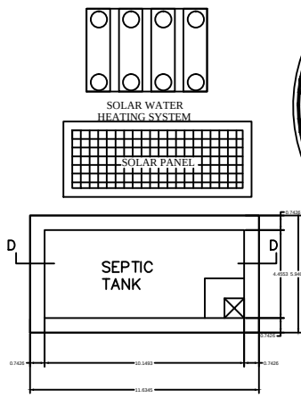
PLAN OF SEPTIC TANK SCALE 1"=2'0"
