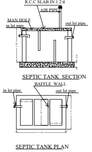
SEPTIC TANK PLAN
