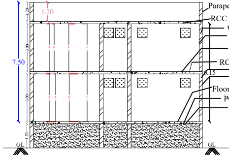
SECTION OF AA
