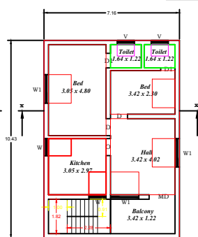
Proposed First Floor Plan
