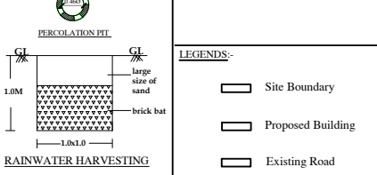
RAINWATER HARVESTING
