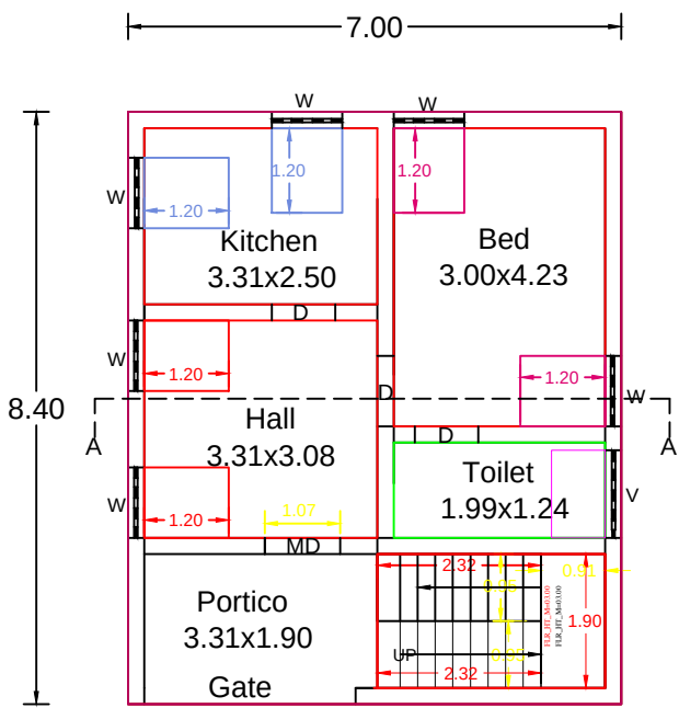
GROUND FLOOR PLAN (Facing North)
