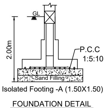
FOUNDATION DETAIL
