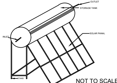
SOLAR WATER HEATER DETAILS
