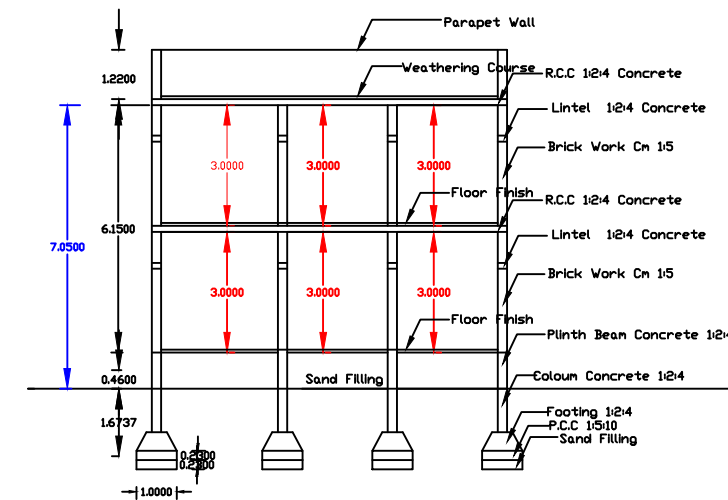
Section Section - AA
