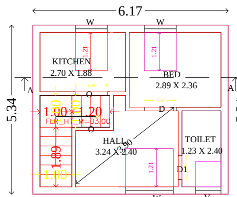
FIRST FLOOR (NORTH FACING)
