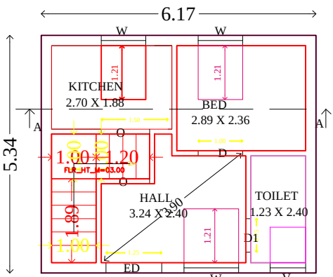
GROUND FLOOR (NORTH FACING)
