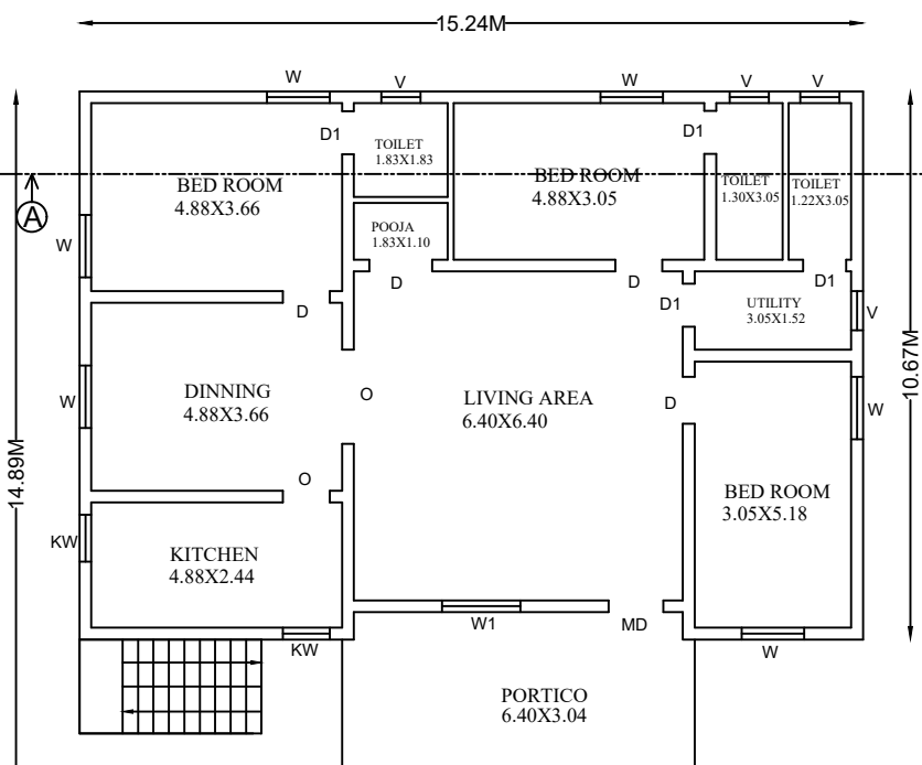
GROUND FLOOR PLAN (RESIDENTIAL)
