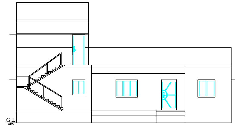
ELEVATION (RESIDENTIAL)
