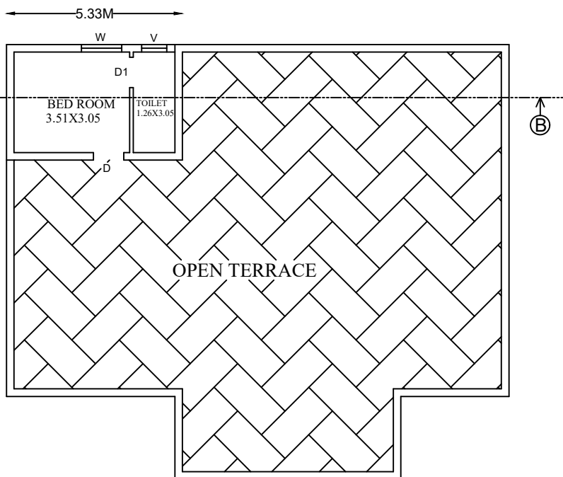
FIRST FLOOR PLAN (RESIDENTIAL)
