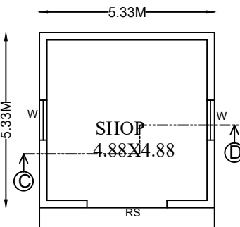
GROUND FLOOR PLAN (COMMERCIAL)
