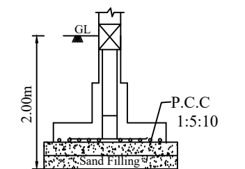
Isolated Footing -A (1.50X1.50)
