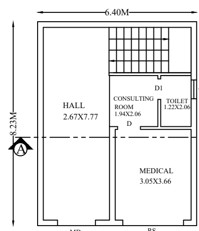
GROUND FLOOR PLAN (COMMERCIAL)
