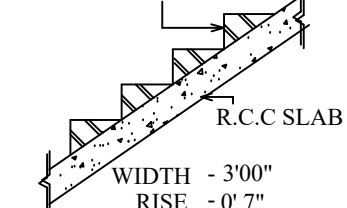
STAIR DETAILS
