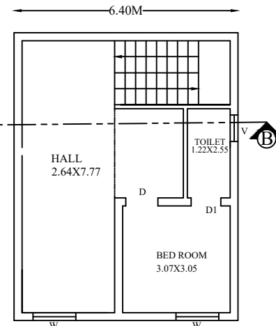
FIRST FLOOR PLAN (RESIDENTIAL)
