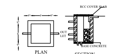
SECTION RAIN WATER COLLECTION PIT DETAILS NOT TO SCALE
