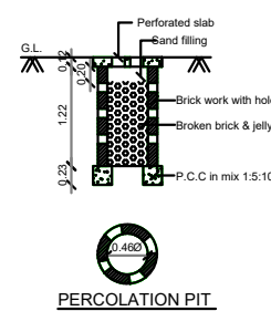
PERCOLATION PIT
