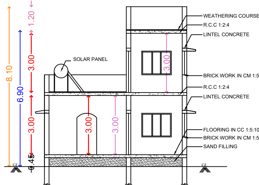
SECTION AB
