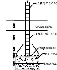
STAIRCASE DETAILS
