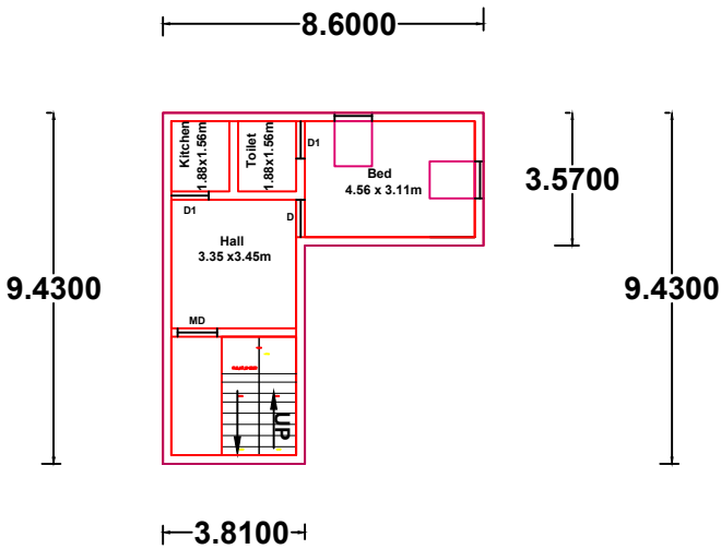
FIRST FLOOR PLAN (PROPOSED)
