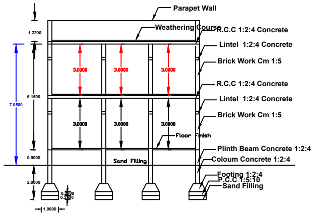
Section Section - AA
