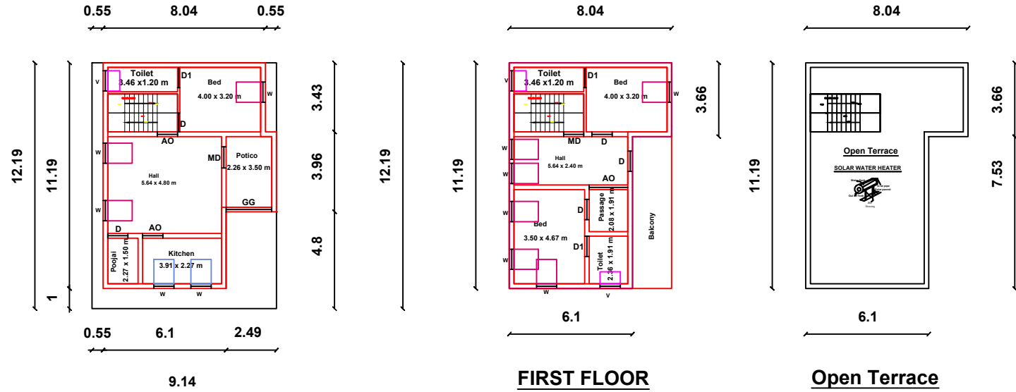
GROUND FLOOR (EAST FACING)
