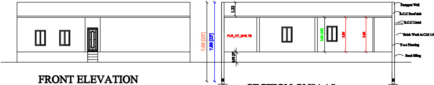
SECTION ON"AA"
