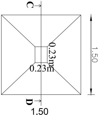
SECTION - 'CD' Plan
