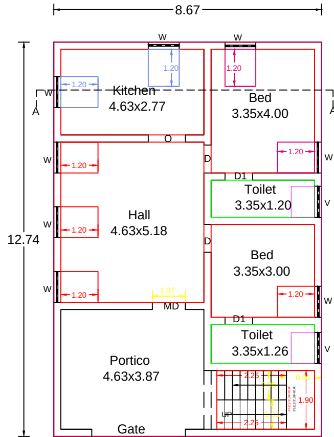
GROUND FLOOR PLAN (Facing North)
