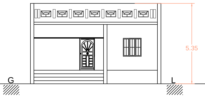
FRONT ELEVATION
