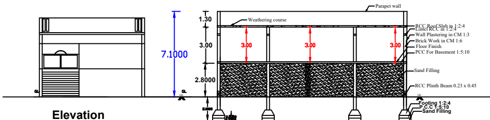
Section Section - AA
