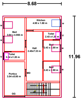
GROUND FLOOR (West Facing)
