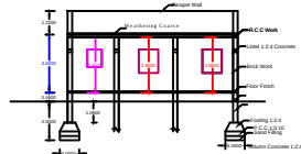
SECTION SECTION - AB
