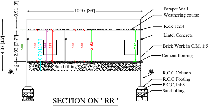
SECTION ON 'RR'
