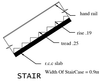
STAIR
