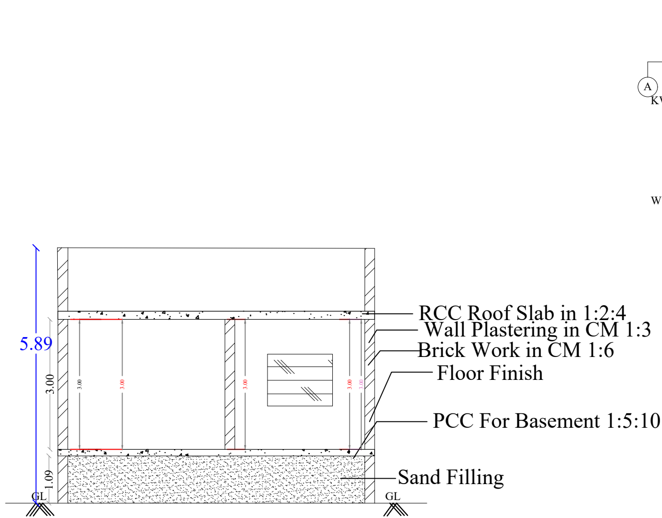
SECTION AA
