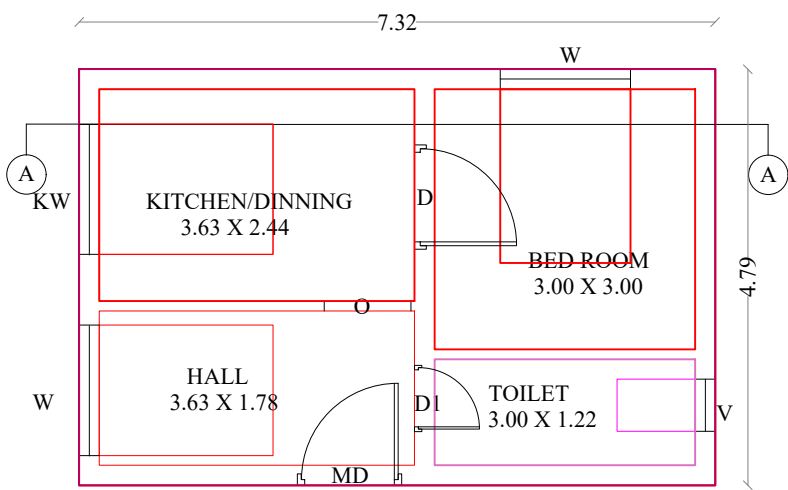
GROUND FLOOR PLAN (NORTH FACING)
