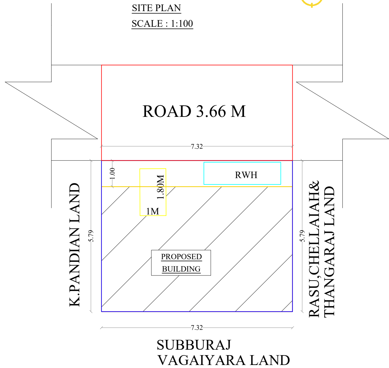
SITE PLAN
