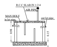
SEPTIC TANK DETAILS
