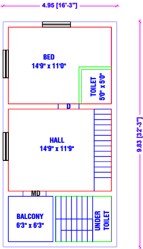
FIRST FLOOR PLAN [NORTH FACING]
