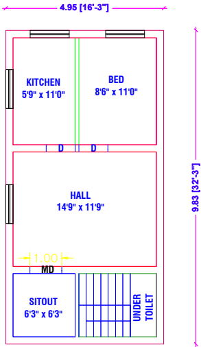
JND FLOOR PLAN [ORTH FACING]
