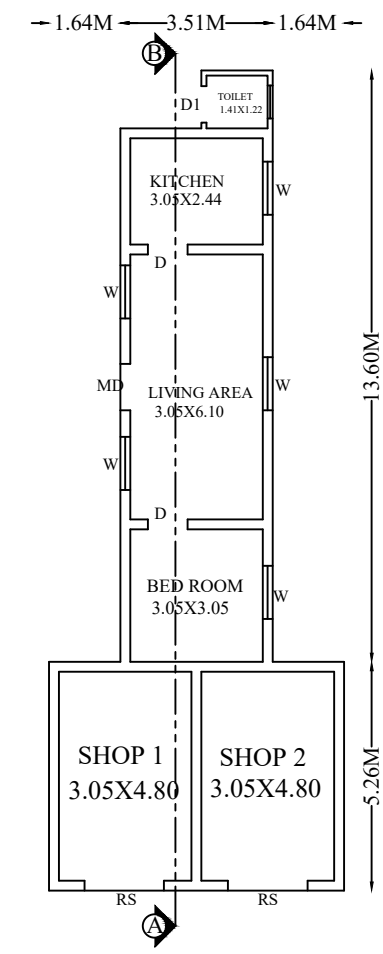
GROUND FLOOR PLAN (COMMERCIAL)
