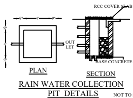
RAIN WATER COLLECTION PIT DETAILS
