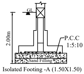
FOUNDATION DETAIL
