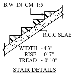
STAIR DETAILS
