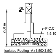
FOUNDATION DETAIL - A
