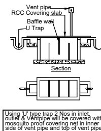
SEPTIC TANK WITH U TRAP
