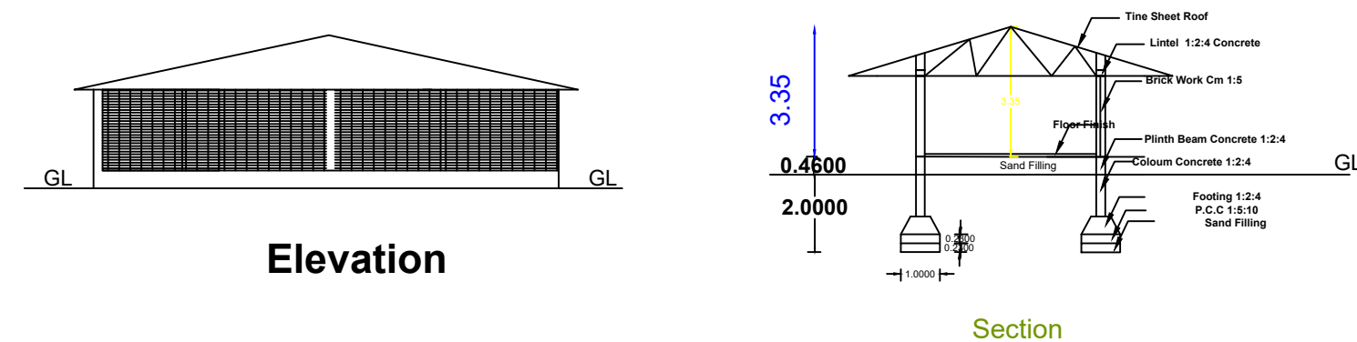
Section - AA
