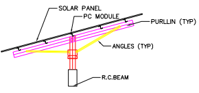
SOLAR PANELS SECTION X-X
