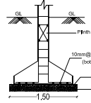
SECTION FOUNDATION DETAILS
