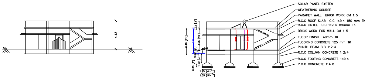
FRONT ELEVATION
