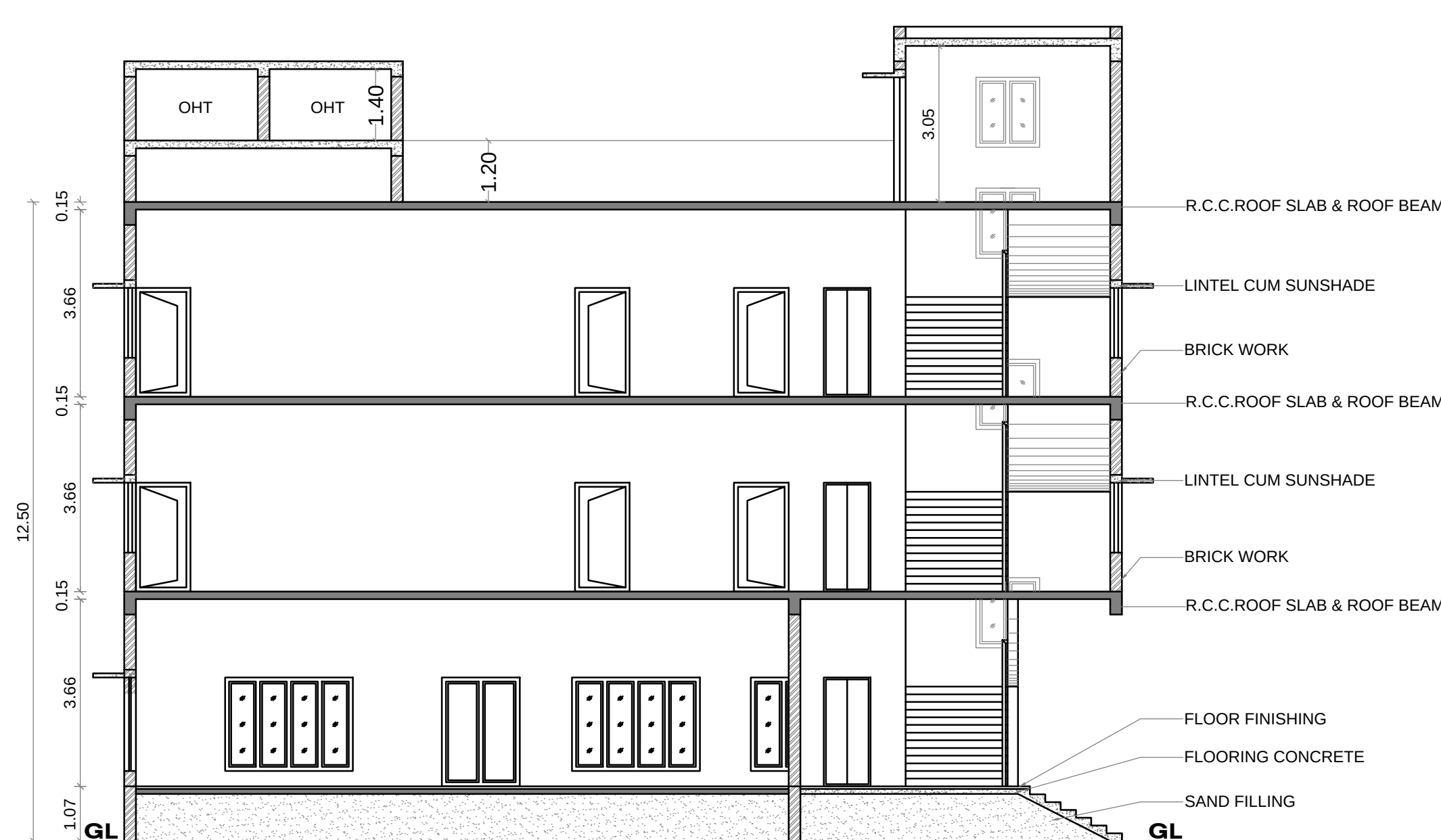
BLOCK-I SECTION - "AA"
