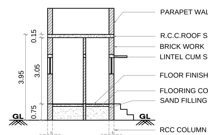
BLOCK -II SECTION - "BB"
