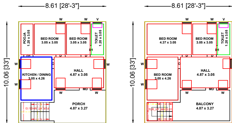
GROUND FLOOR PLAN (EAST FACING)
