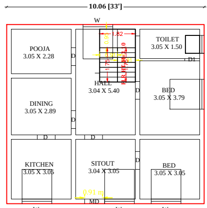
GROUND FLOOR PLAN EAST FACING
