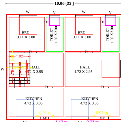
FIRST FLOOR PLAN EAST FACING
