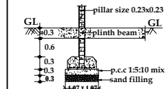
FOUNDATION DETAILS
