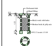
PERCOLATION PIT
