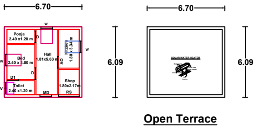
GROUND FLOOR
