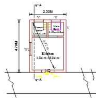
GROUND FLOOR PLAN [NORTH FACING]
