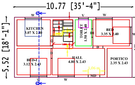
GROUND FLOOR PLAN (NORTH FACING)
