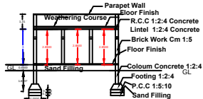
Section Section - AB
