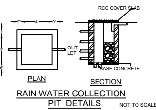
RAIN WATER COLLECTION PIT DETAILS
