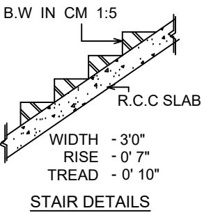
STAIR DETAILS
