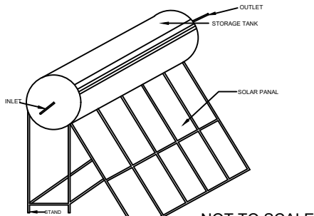
NOT TO SCALE SOLAR WATER HEATER DETAILS
