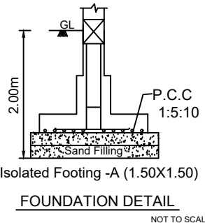
FOUNDATION DETAIL
