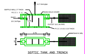
SEPTIC TANK AND TRENCH
