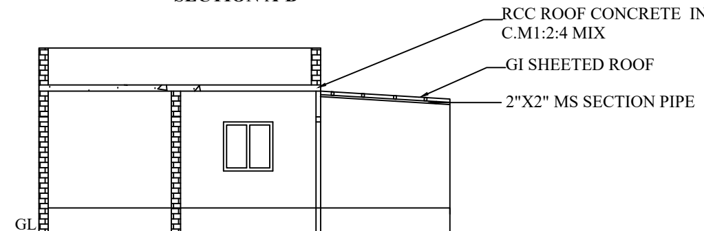
SECTION X-Y
