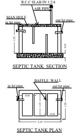
SEPTIC TANK PLAN
