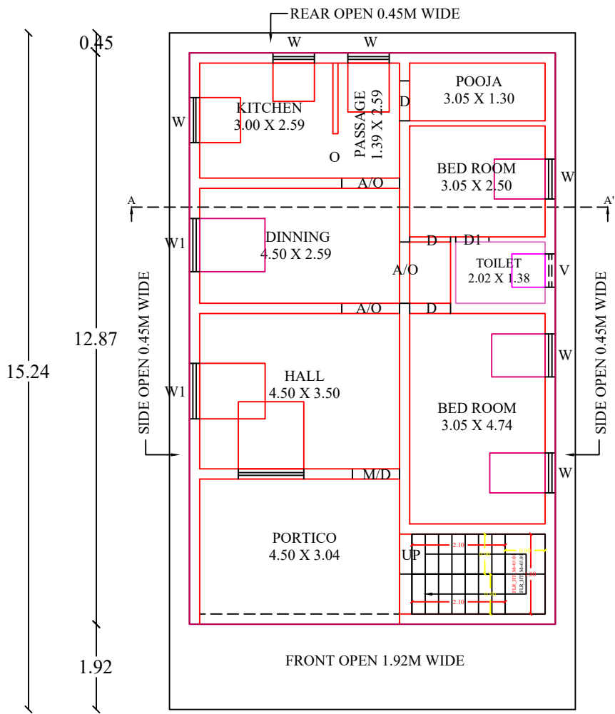
GROUND FLOOR PLAN (NORTH FACING)
