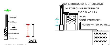
RAINWATER HARVESTING
