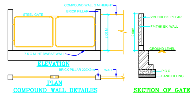
SECTION OF GATE
