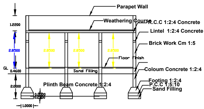
Section Section - AA
