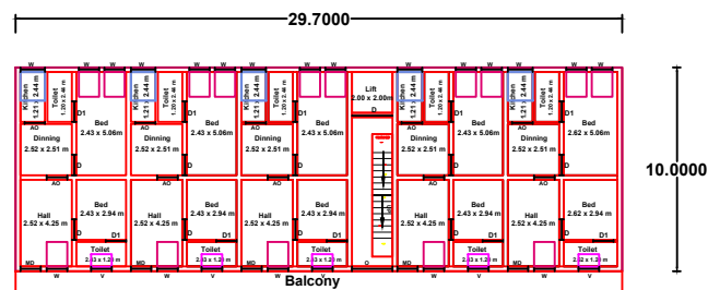
PROPOSED FIRST FLOOR (NORTH FACING)
