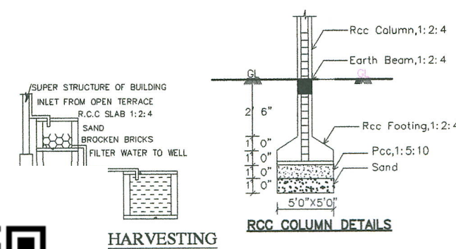
RCC COLUMN DETAILS
