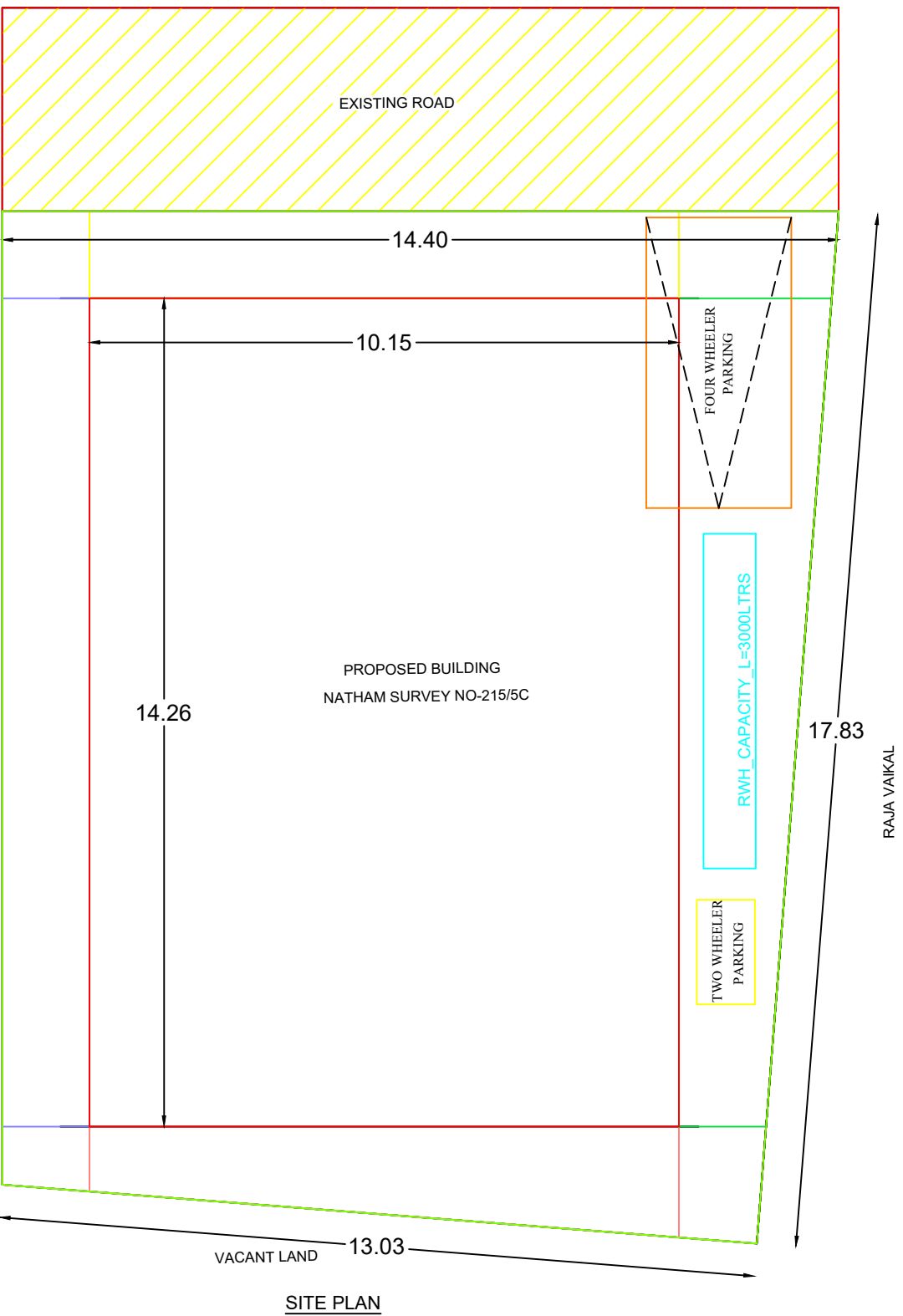
SITE PLAN
