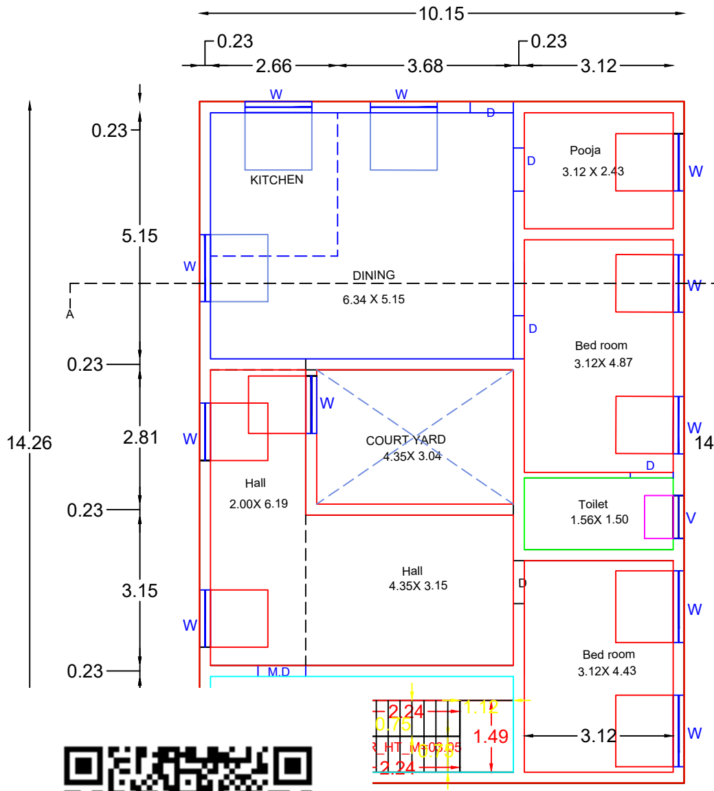
SED GROUND FLOOR PLAN
