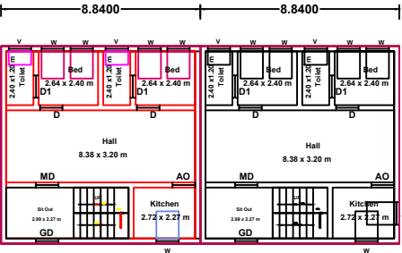
Ground Floor Existing & Proposed Ground Floor
