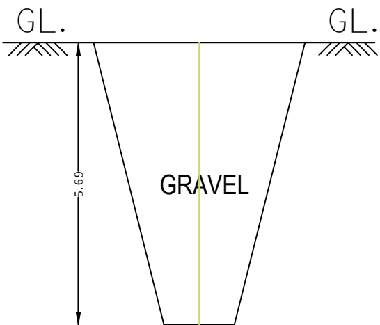
TRIAL PIT
