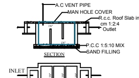
PLAN DETAILS OF SEPTIC TANK (Not to scale)
