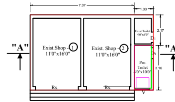
EXIST. GROUND FLOOR AND EXTENSION OF TOILET PLAN
