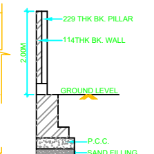
SECTION OF GATE
