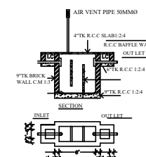
PLAN SEPTIC TANK DETAILS SCALE 1"=8'0"
