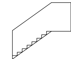
Stair HAND RAIL = 1.00M STAIR WIDTH = 0.90M RAISER = 0.18M TREAD = 0.25M
