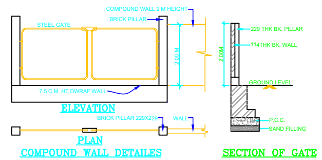
SECTION OF GATE
