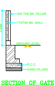
SECTION OF GATE
