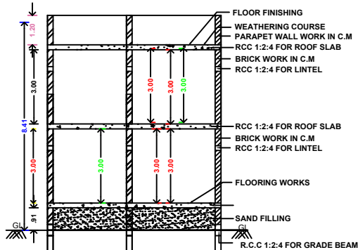
SECTION ON "BB"
