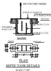
SEPTIC TANK DETAILS
