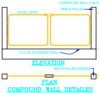
COMPOUND WALL DETAILS
