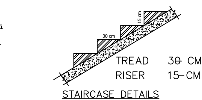
STAIRCASE DETAILS
