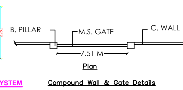
Compound Wall & Gate Details
